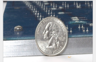
Beveled design of the 3/8" Bashplate protects LEDs and internal components by dissipating any force inflicted on the sign.
